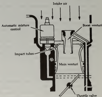
FIGURE 3-21. Automatic mixture control and throttle body.
